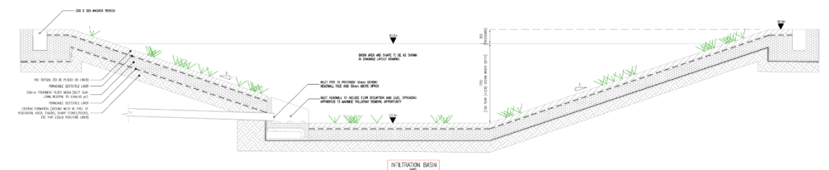
Plate 5.33 – Infiltration basin – image 2 (not to scale)
