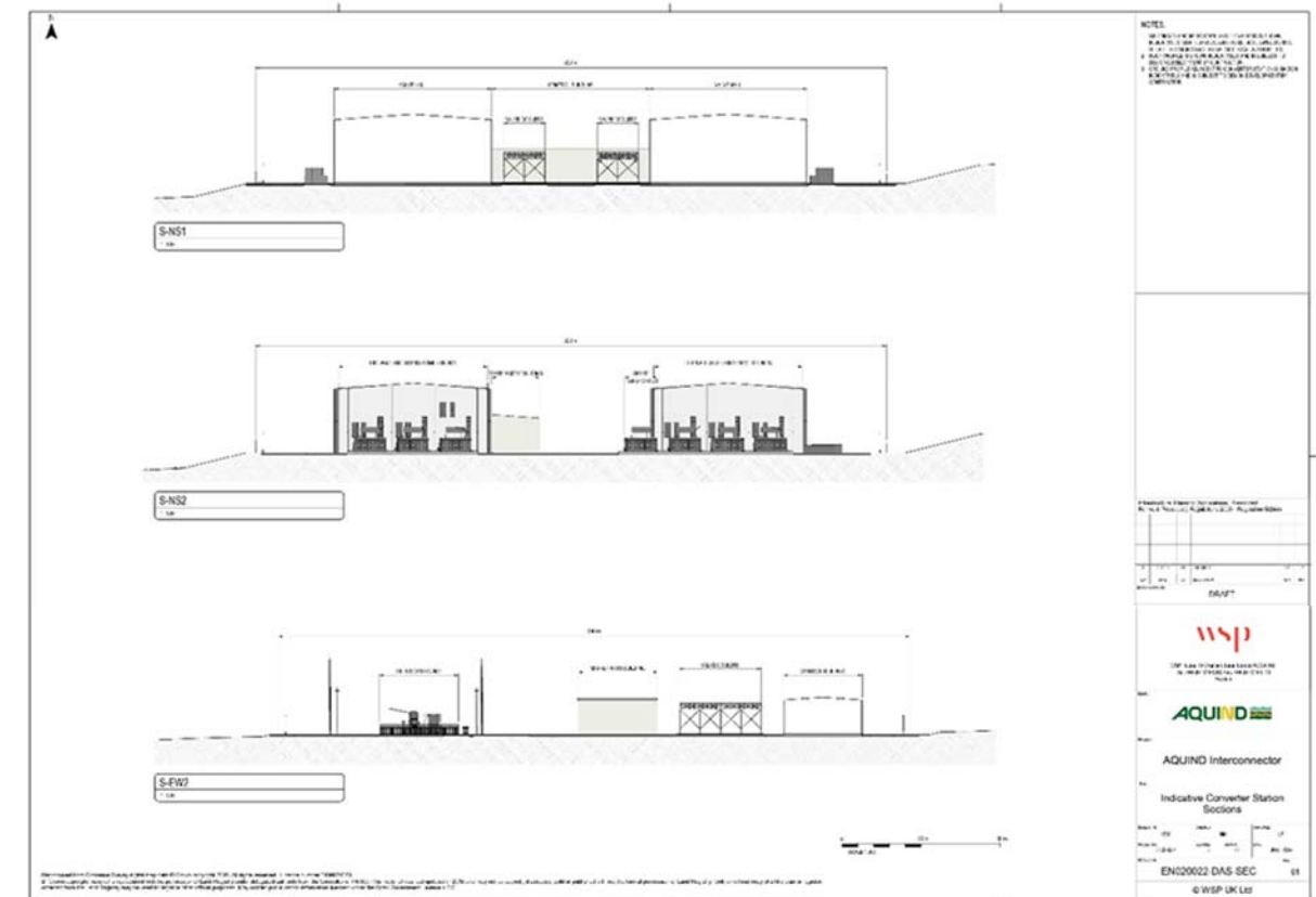
Plate 7.6 Indicative Converter Station Sections
