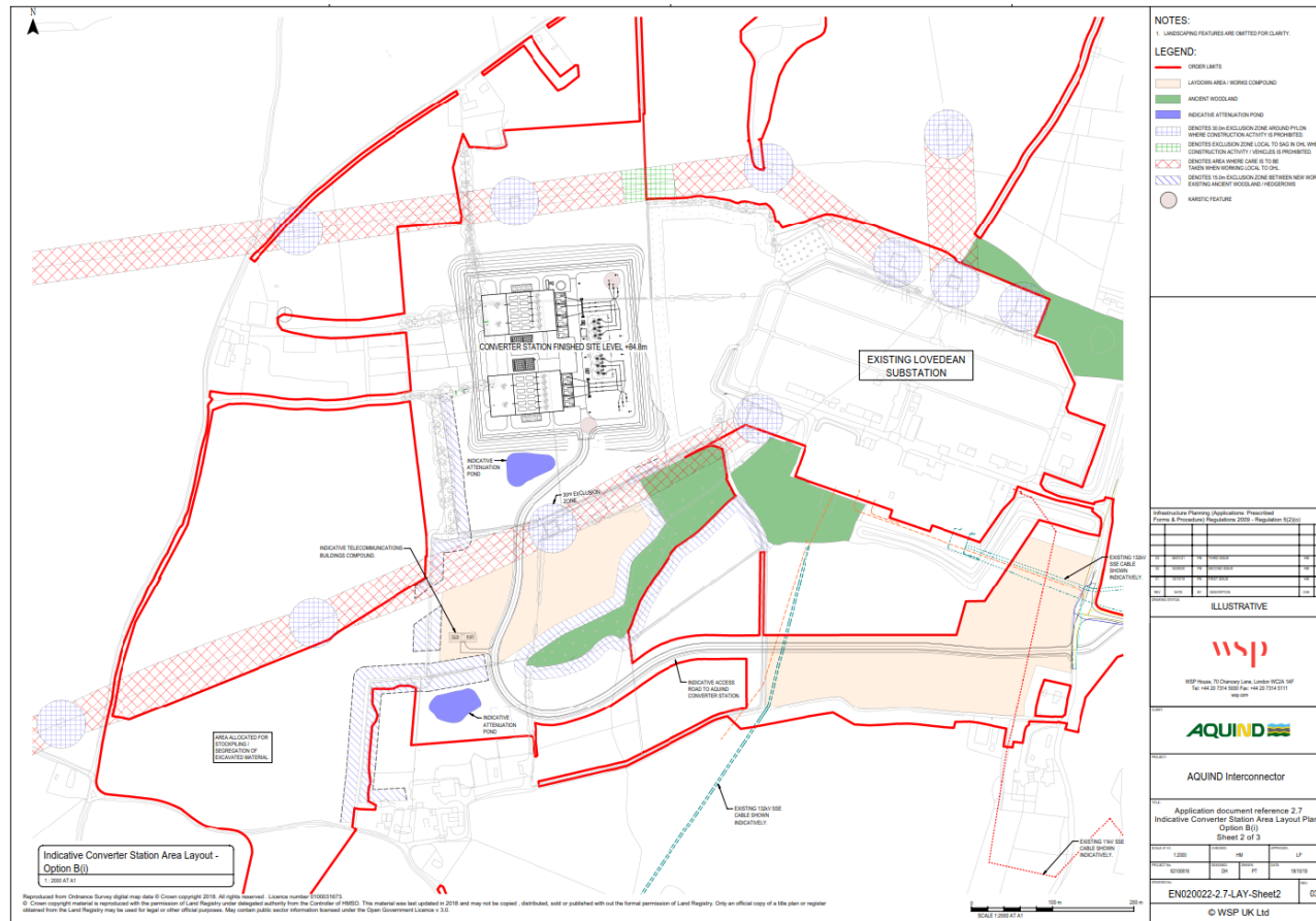
Plate 5.3 – Indicative site layout (Option B (i)) [APP-013]: illustrating the location of the compound defined by the Parameter Plans and how the access to it could be arranged to preserve the ancient woodland and land ownership constraints.
