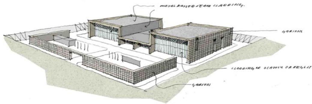
Options 1 – Gabion
